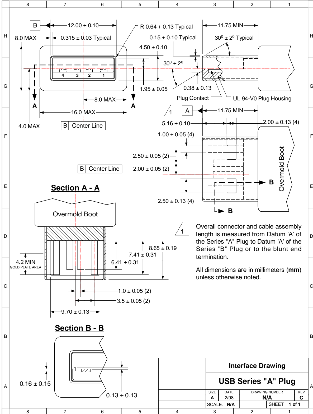
Figure 6-9 Figure 6-13. USB Series "A" Plug Interface Drawing
